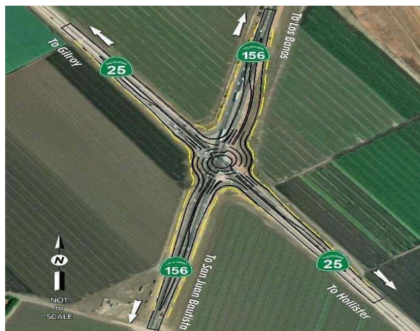
Figure 4-2: SR25/SR156 Turbo Roundabout
